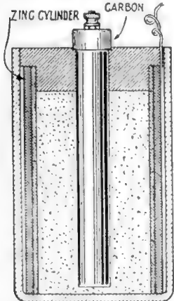
A Home-made dry battery cell
